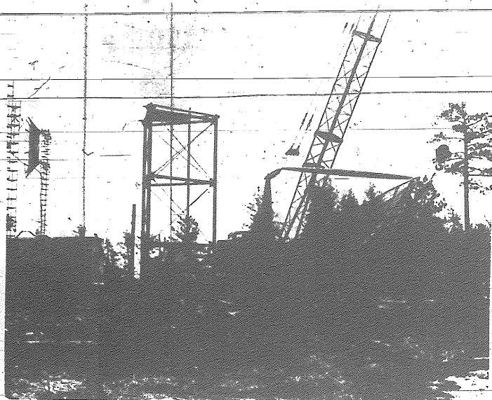
Two years ago Norwesto installed the first Tropospheric Scatter system between Kenora and Red Lake. Two huge antennae (or dishes) were erected, one at each end, to receive signals. Several weeks ago these were replaced with even larger "dishes." Photos, taken at the top of Mellick Av.
