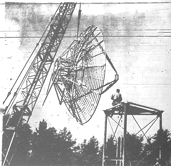
ene hill in Kenora show (1) the new "dish" on the ground with the smaller one pointing north, which was being replaced. (2) the "dish" half-way to its stand on the end of an 80 foot boom; (3) just about there.
